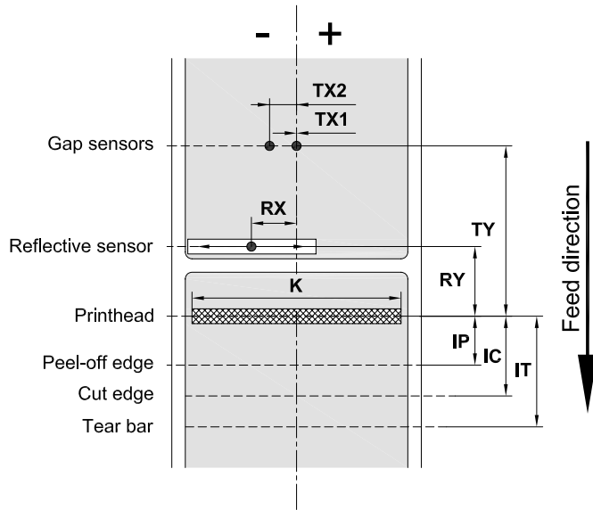
Fig. 12 Device dimensions
