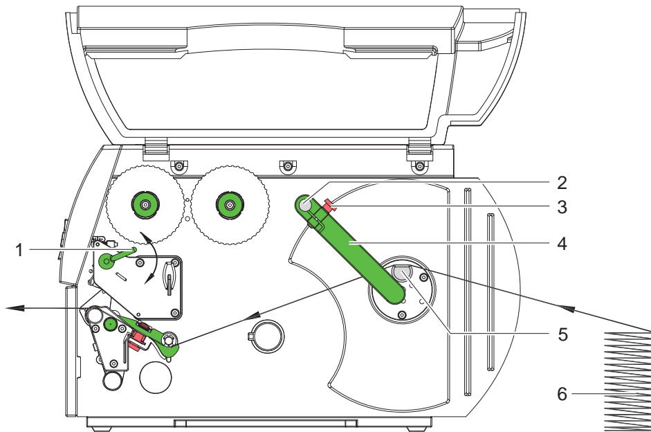
Fig. 8 Feed path of fanfold labels
