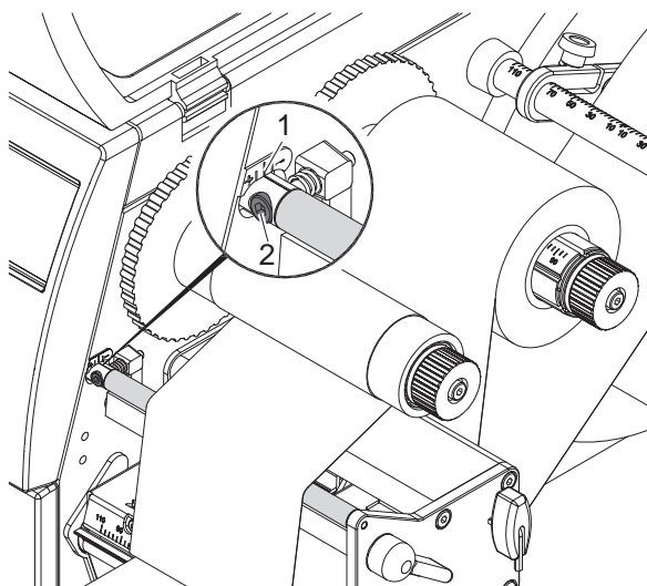
Fig. 11 Setting the feed path of the transfer ribbon
