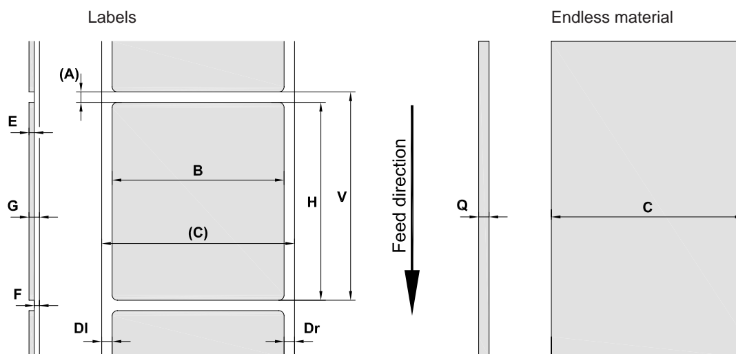
Fig. 13 Label / endless material dimensions
