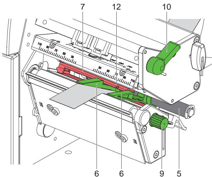
Fig. 7 Inserting a Media Strip into the Printhead
