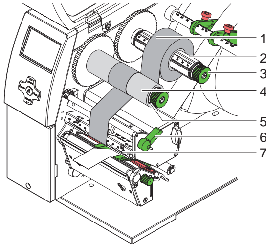
Fig. 9 Load transfer ribbon
