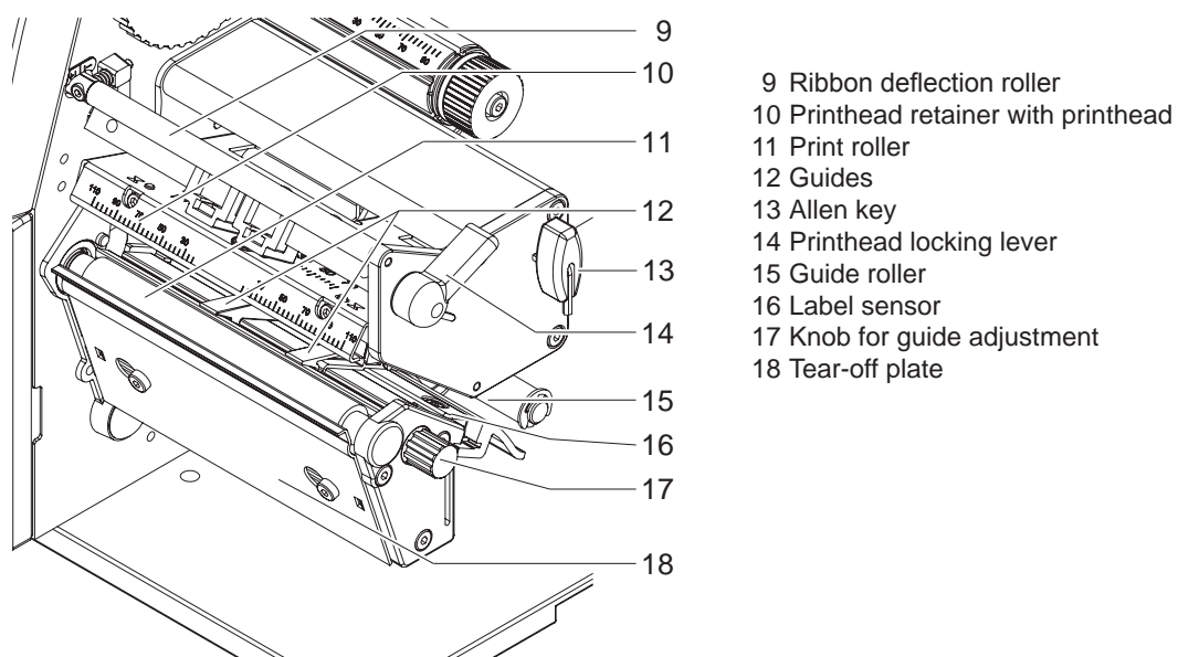
Fig. 2 Print mechanics
