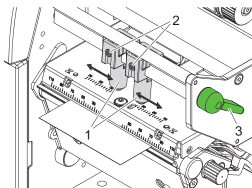
Fig. 12 Setting the head locking system
