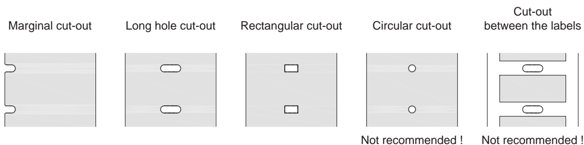
Fig. 17 Samples for cut-out marks
