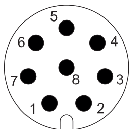
Connector pin assignment
