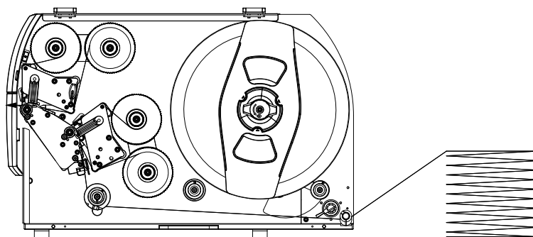
Label feed path
