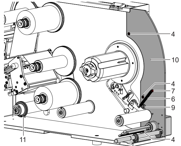
Assembly the fanfold guide
