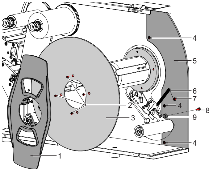
Dismounting the standard fin
