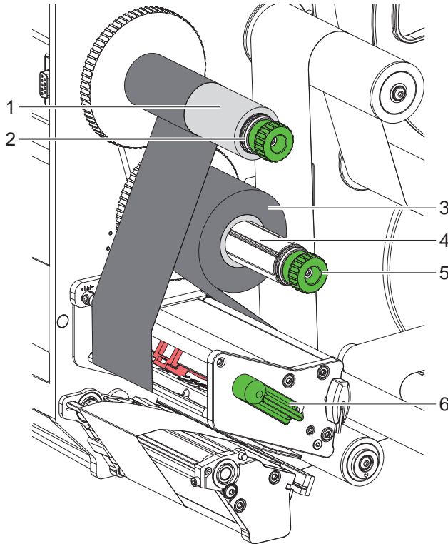
Figure 18 Insertion du ruban transfert
