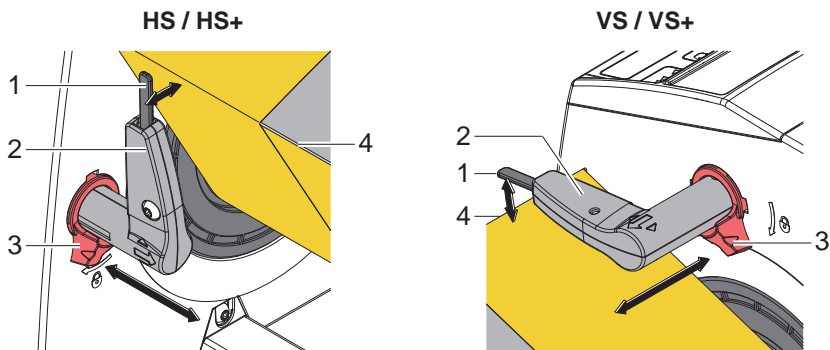
Fig. 7 Adjusting the present sensor
