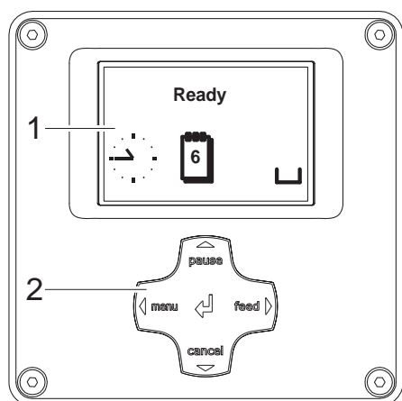
Fig. 7 Control Panel
