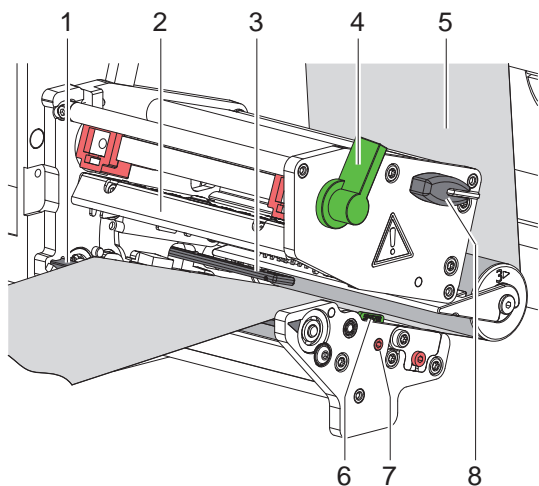
Fig. 10 Inserting the labels into the print mechanism
