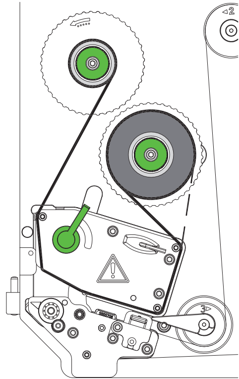
Fig. 16 Transfer ribbon feed path
